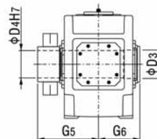
H2DH, H2DM 带胀紧盘的空心轴 Hollow shaft for shrink disk
