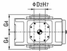
B2HV 空心轴 Hollow shaft
