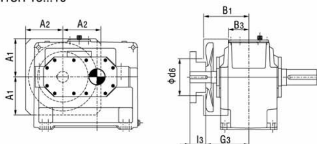
H1SH 13...19
