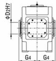
H2HH, H2HM 空心轴 Hollow shaft
