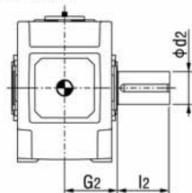
B2SH 实心轴 Solid shaft
