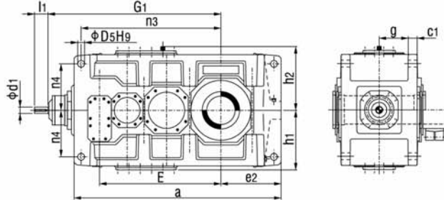
B4HM, B4DM
