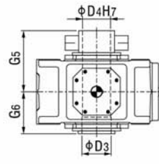
B3DV 带胀紧盘的空心轴 Hollow shaft for shrink disk
