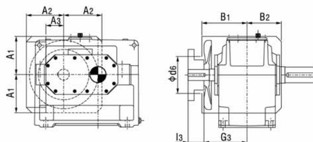
H1SH 3 ... 11
