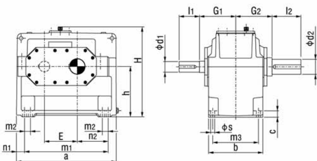
H1SH
