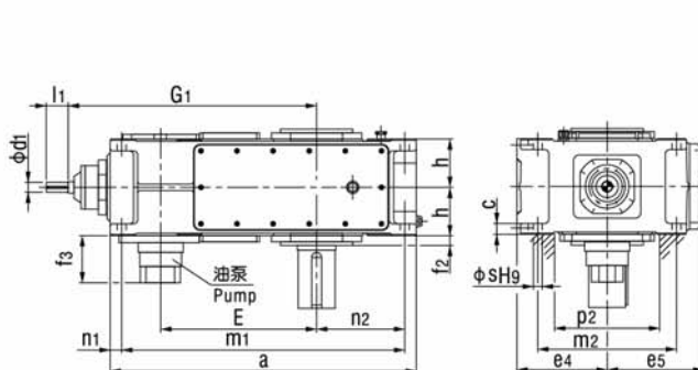
B4SV、B4HV、B4DV (强制润滑 With forced lubrication)
