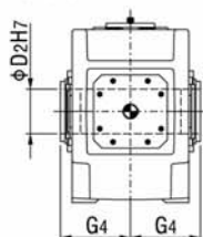
B4HH, B4HM 空心轴 Hollow shaft
