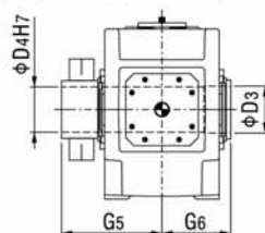
B4DH, B4DM 带胀紧盘的空心轴 Hollow shaft for shrink disk
