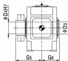
B2DH, B2DM 带胀紧盘的空心轴 Hollow shaft for shrink disk
