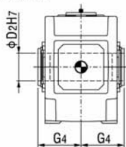
B2HH, B2HM 空心轴 Hollow shaft
