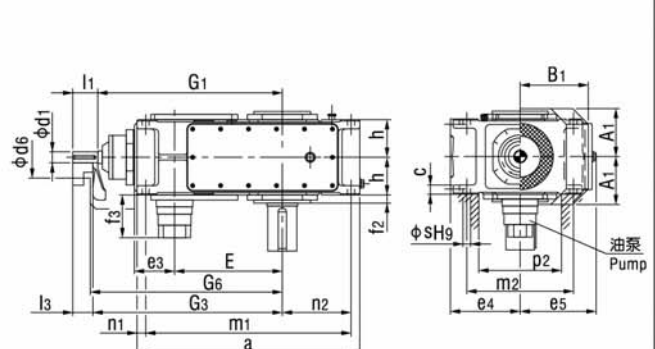
B3SV、B3HV、B3DV (强制润滑 With forced lubrication)
